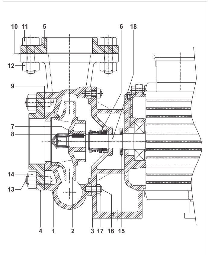
FIG.1 SECTIONAL DRAWING OF LBI PUMP
